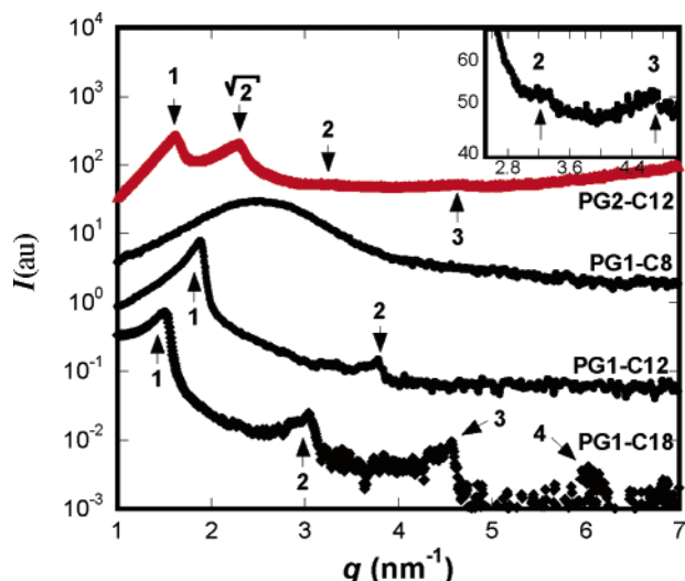
Figure 1. SAXS diffractograms for PG1 (three lowest curves) and PG2 (upper and inset curves) dendronized polymers complexed with C8, C12, and C18. Multiple reflections are indexed by arrows. The PG2 –C12 spectrum (zoomed in the inset in the 2.5–5 nm -1 region) is given in I \times q^2 .
