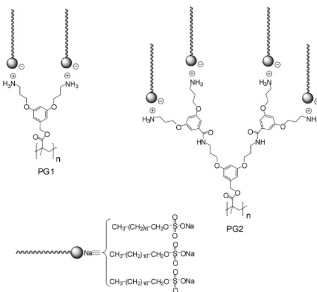
Scheme 1. Complexes of Dendronized Polymers and Surfactants Used
