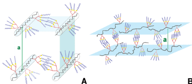
Figure 2. Schematic representation of (A) tetragonal columnar phase and (B) lamellar phase obtained for PG2 –C12 and PG1 –C12 dendronized polymer–surfactant complexes, respectively (see Supporting Information).
